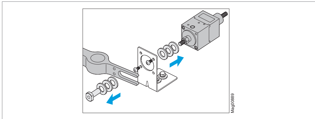
Fig. 60: Remove magnet, washers and union nut
