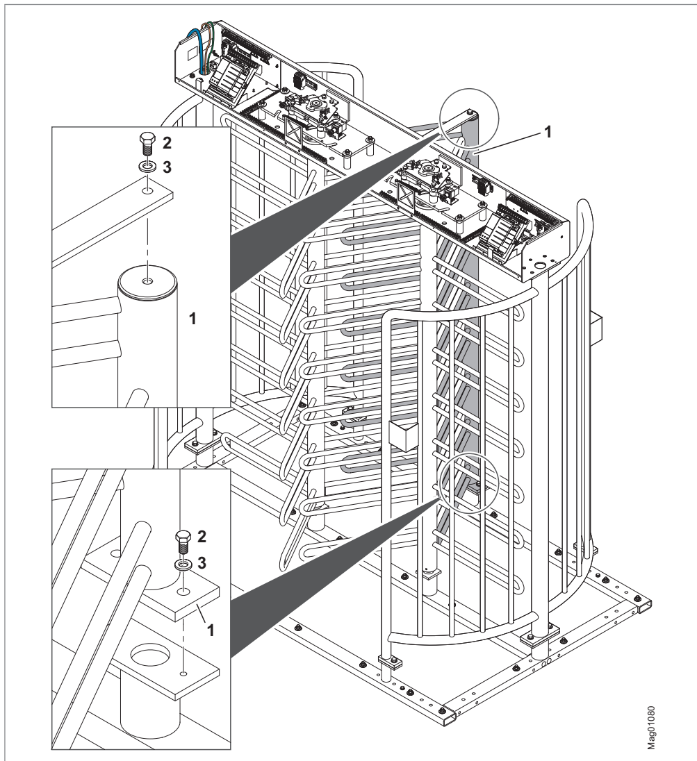
Fig. 41: Mounting the first locking comb
