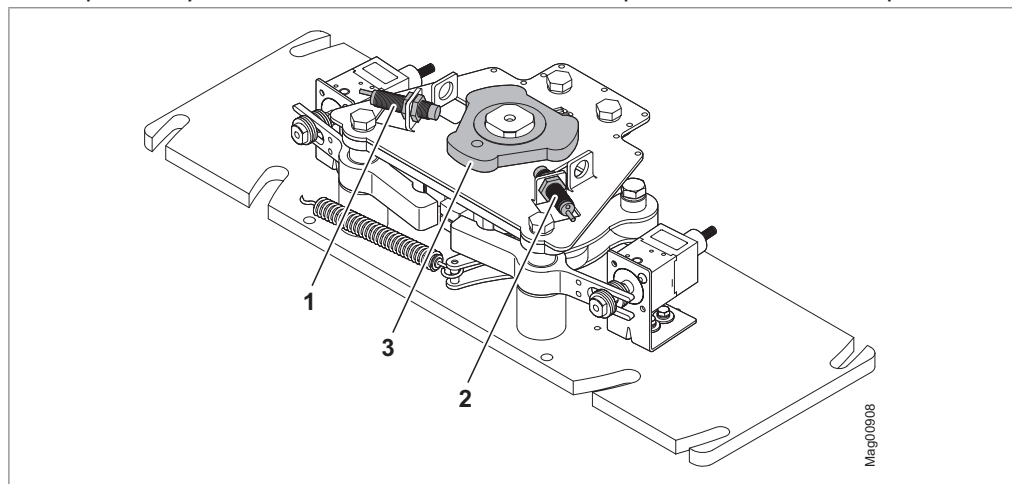
Fig. 56: Proximity sensors for detecting the end position of the centre pillar
