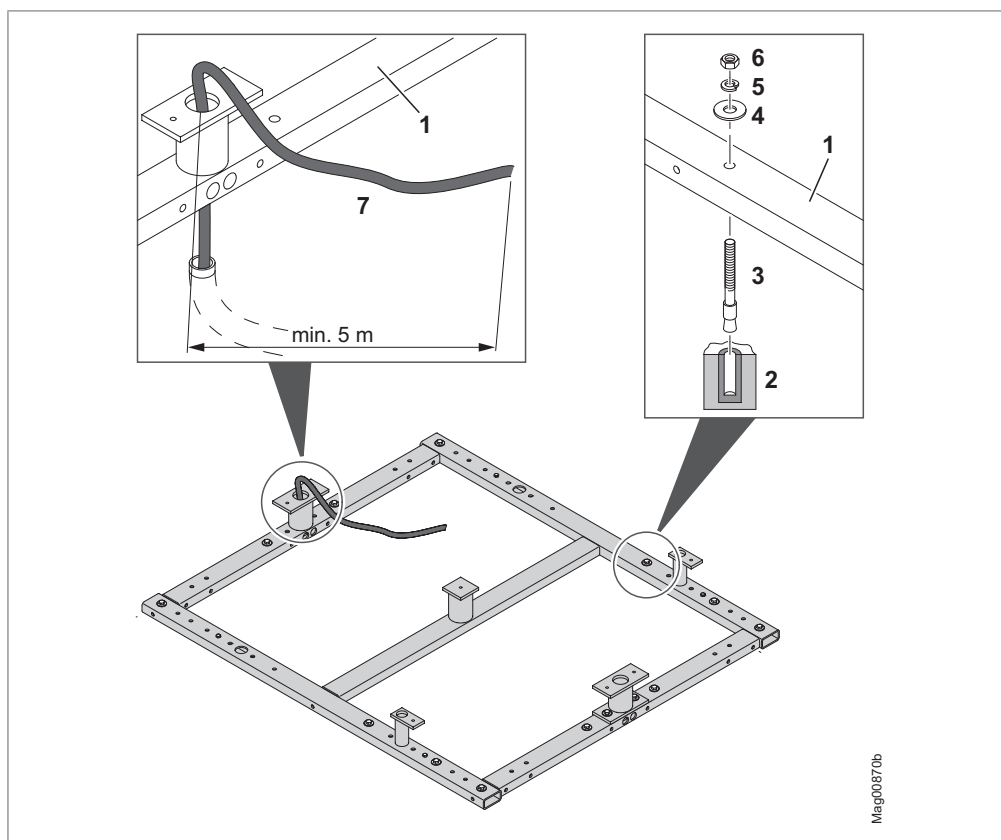
Fig. 21: Assembling the base frame FURA T3
