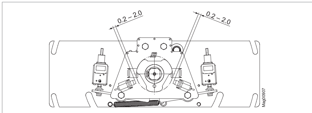
Fig. 57: Distance proximity sensor - switching cam
