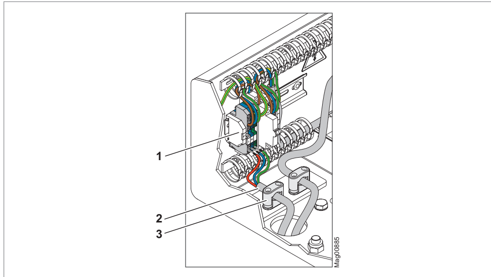
Fig. 54: Connecting the mains cable
