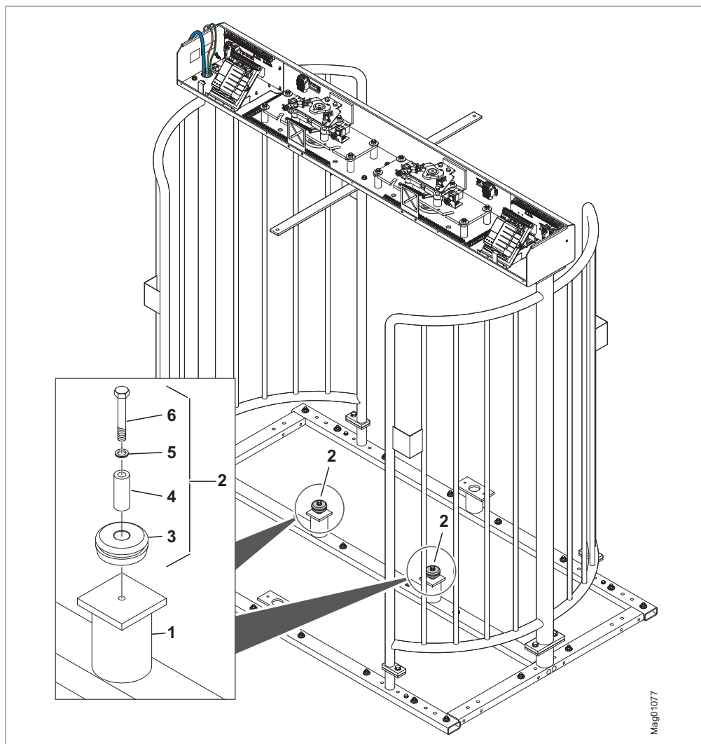
Fig. 37: Mounting the floor bearing (plastic bearing, sleeve, washer and hexagon head screw)
