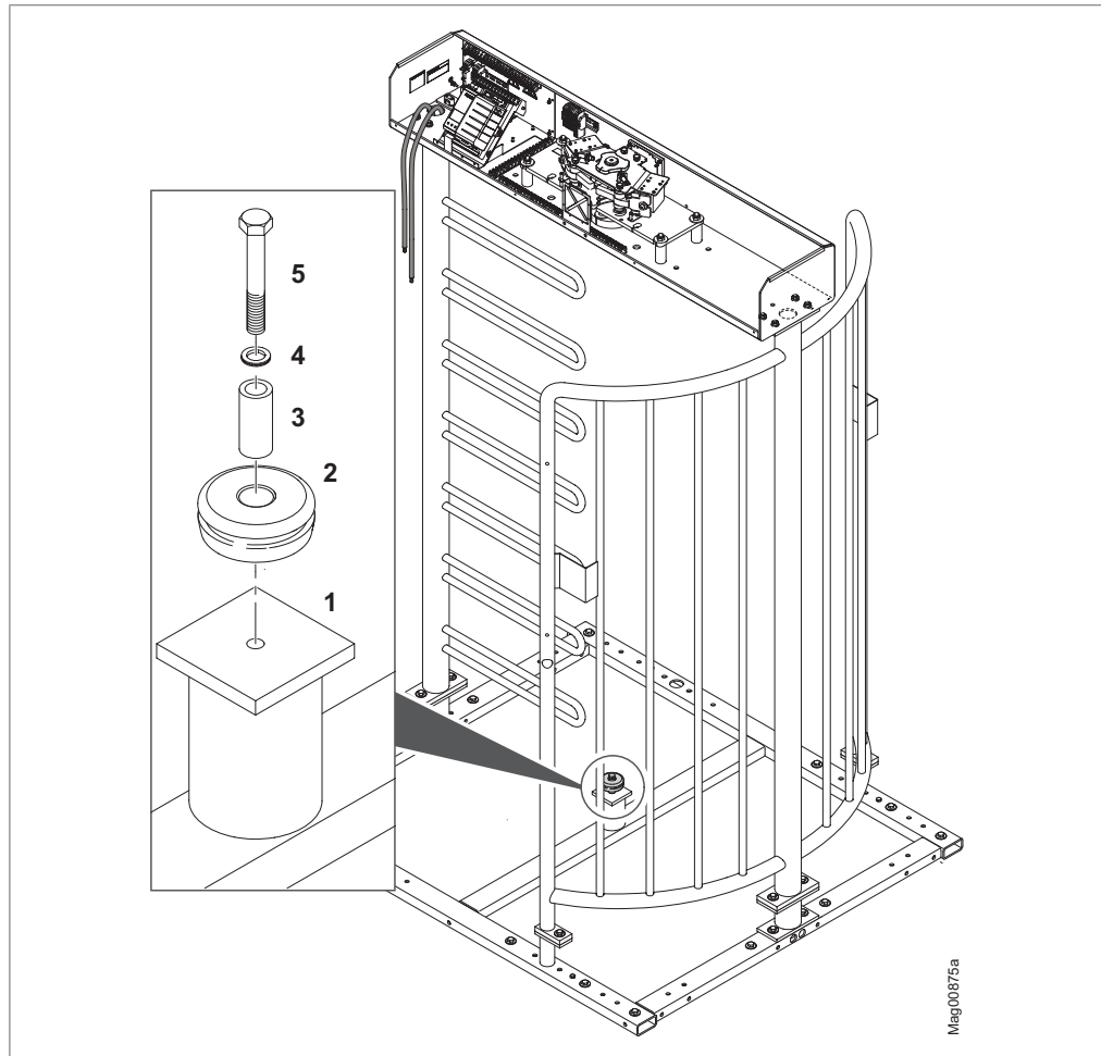
Fig. 25: Mounting the floor bearing (plastic bearing, sleeve, washer and hexagon head screw)
