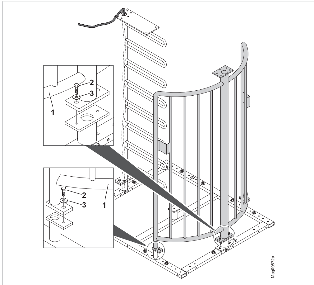
Fig. 23: Mounting the cage half
