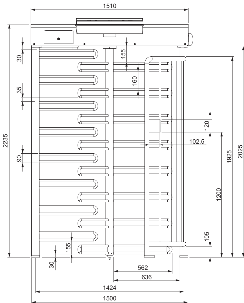
Fig. 1: Dimensions MPT-333 – front view (dimensions in mm), shown here version "entrance side left", illumination optional
