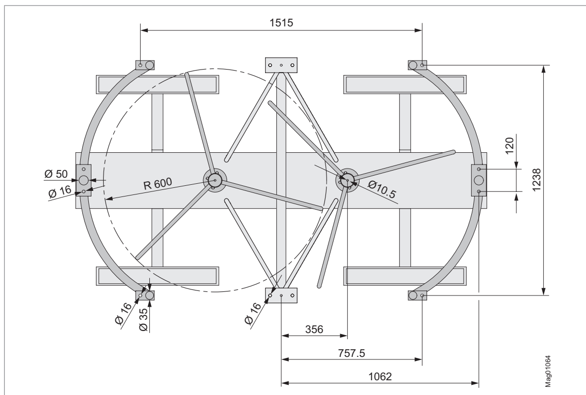
Fig. 6: Dimensions MPT-353 – view from below (dimensions in mm), illumination optional
