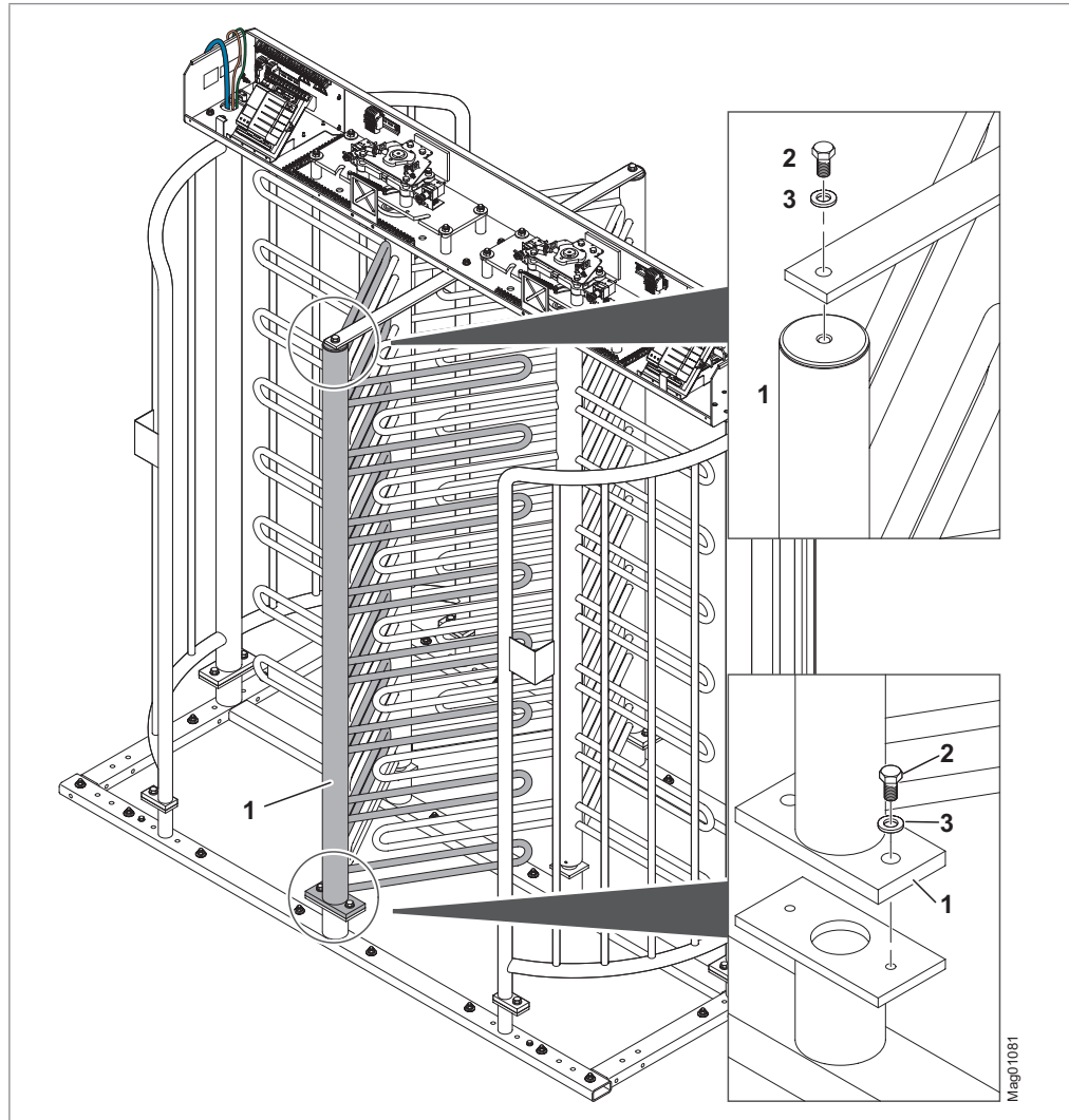
Fig. 42: Mounting the second locking comb
