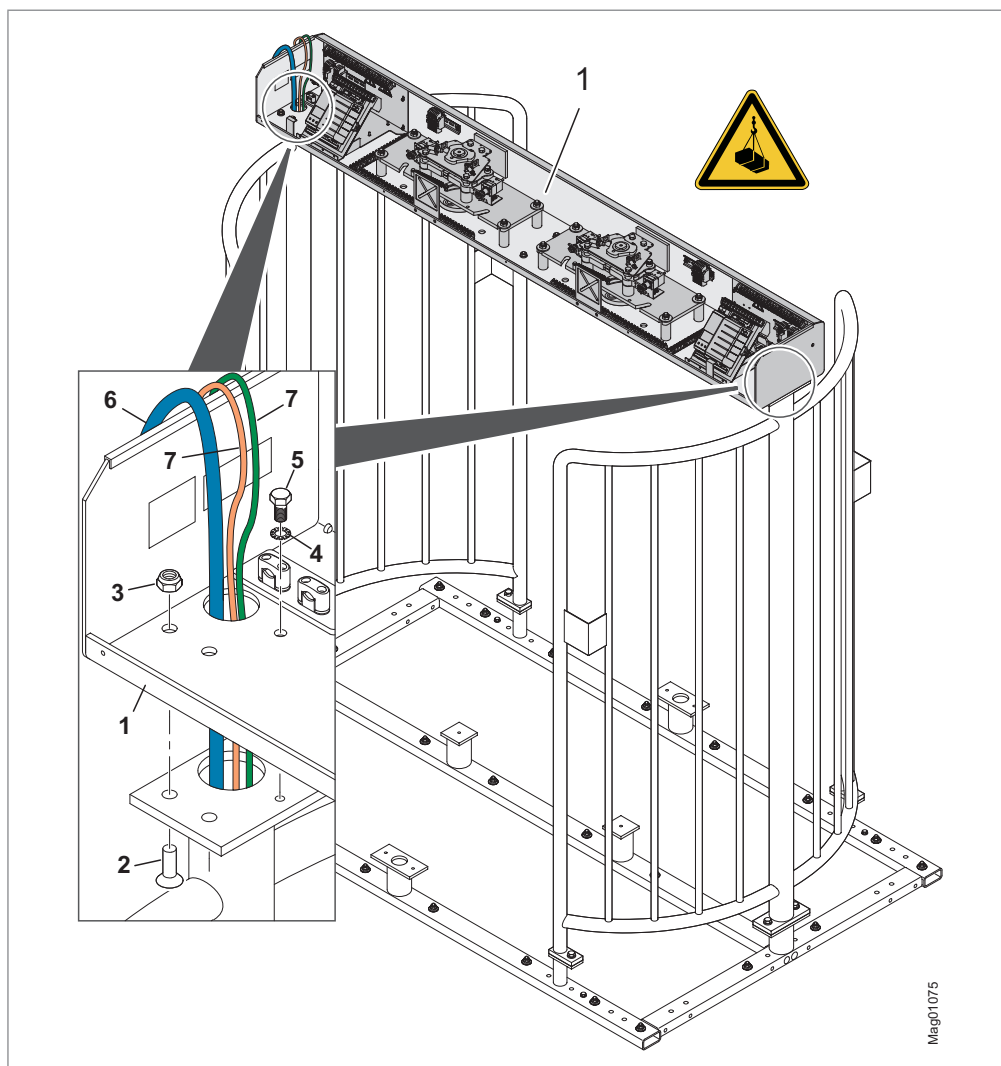
Fig. 35: Putting on the support beam and installing it
