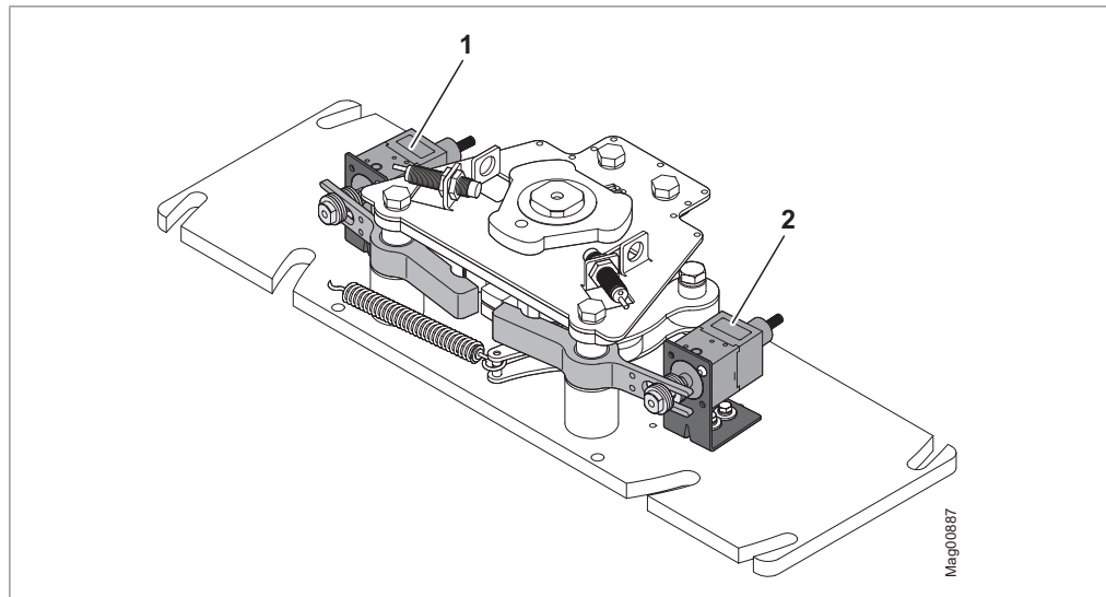
Fig. 58: Locking unit configuration "Normally open"
