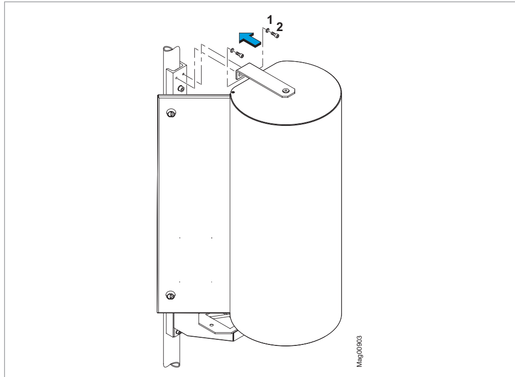
Fig. 49: Mounting the attachment angle
