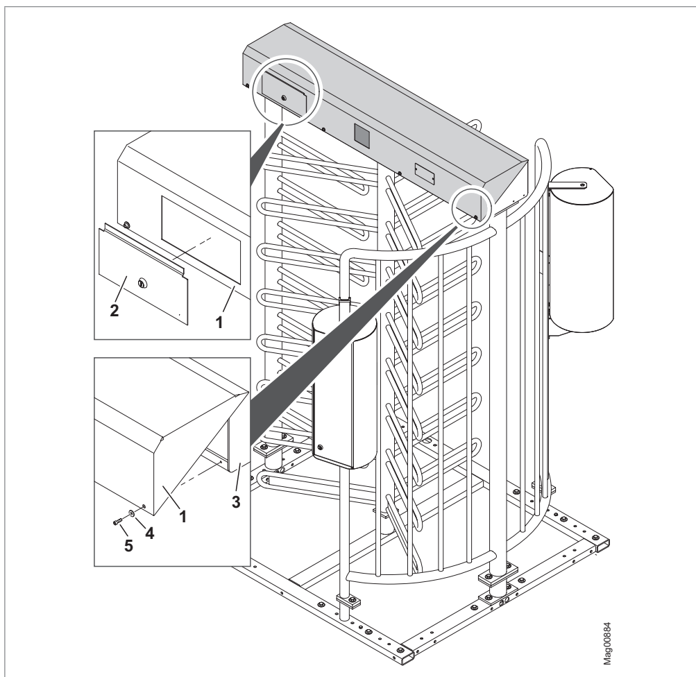
Fig. 52: Open and close cover or service door
