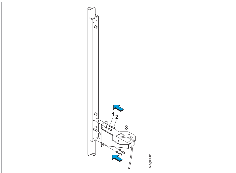
Fig. 47: Mounting the lower holder
