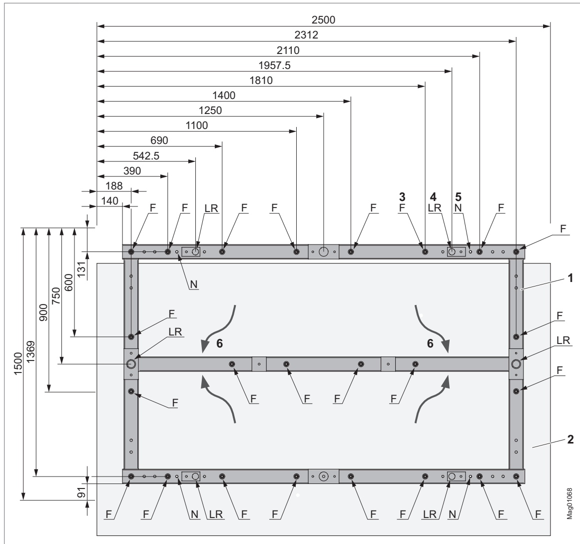
Fig. 28: Foundation and empty conduit plan for base frame FURA T5 – top view (dimensions in mm)
