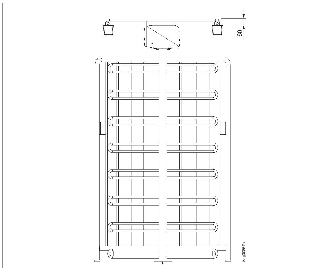
Fig. 2: Dimensions MPT-333 – side view (dimensions in mm), illumination optional
