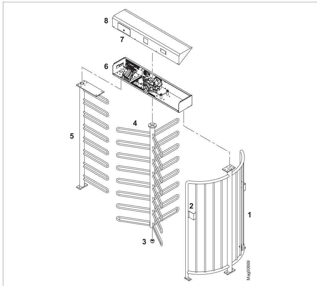
Fig. 7: Design "Full Height Turnstile MPT-333"
