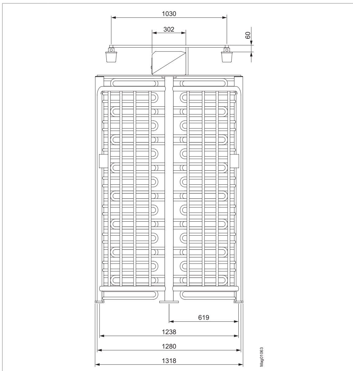
Fig. 5: Dimensions MPT-353 – side view (dimensions in mm), illumination optional
