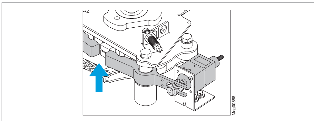
Fig. 59: Locking unit configuration "Normally open"
