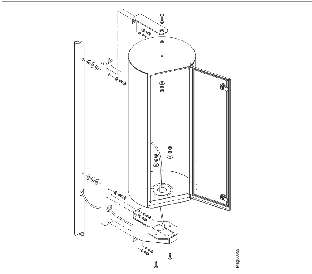
Fig. 45: Mounting pillar and attachment material
