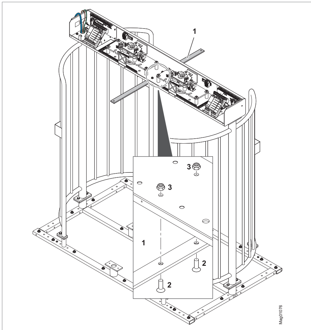
Fig. 36: Mounting the connecting rod
