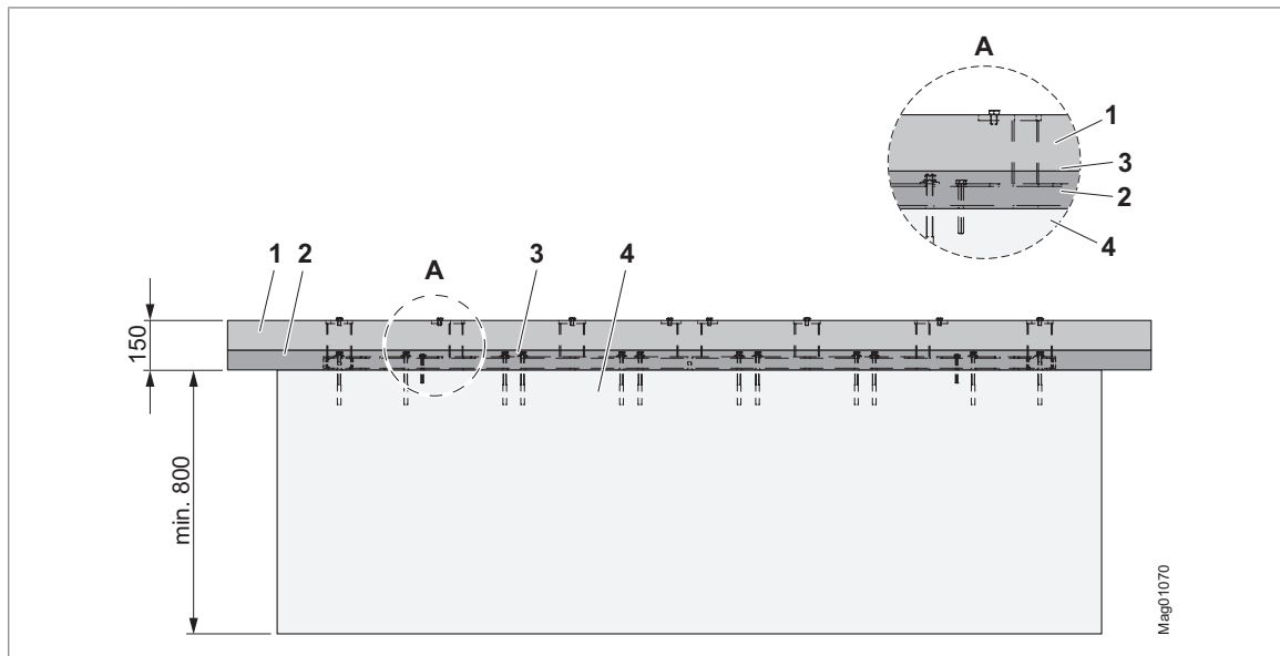
Fig. 29: Foundation and empty conduit plan for base frame FURA T5 – side view (dimensions in mm)
