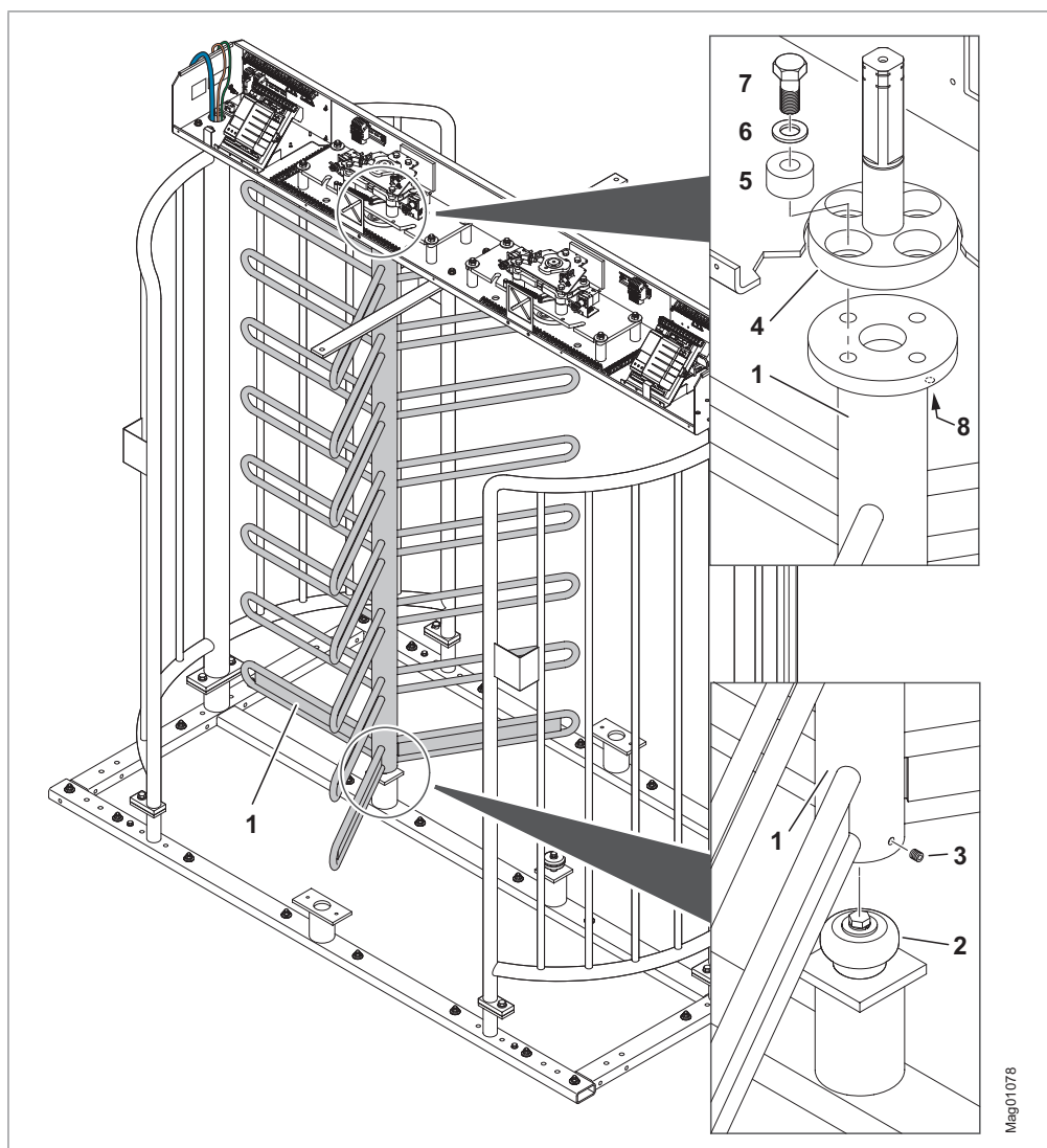
Fig. 38: Mounting centre pillar with heel guard
