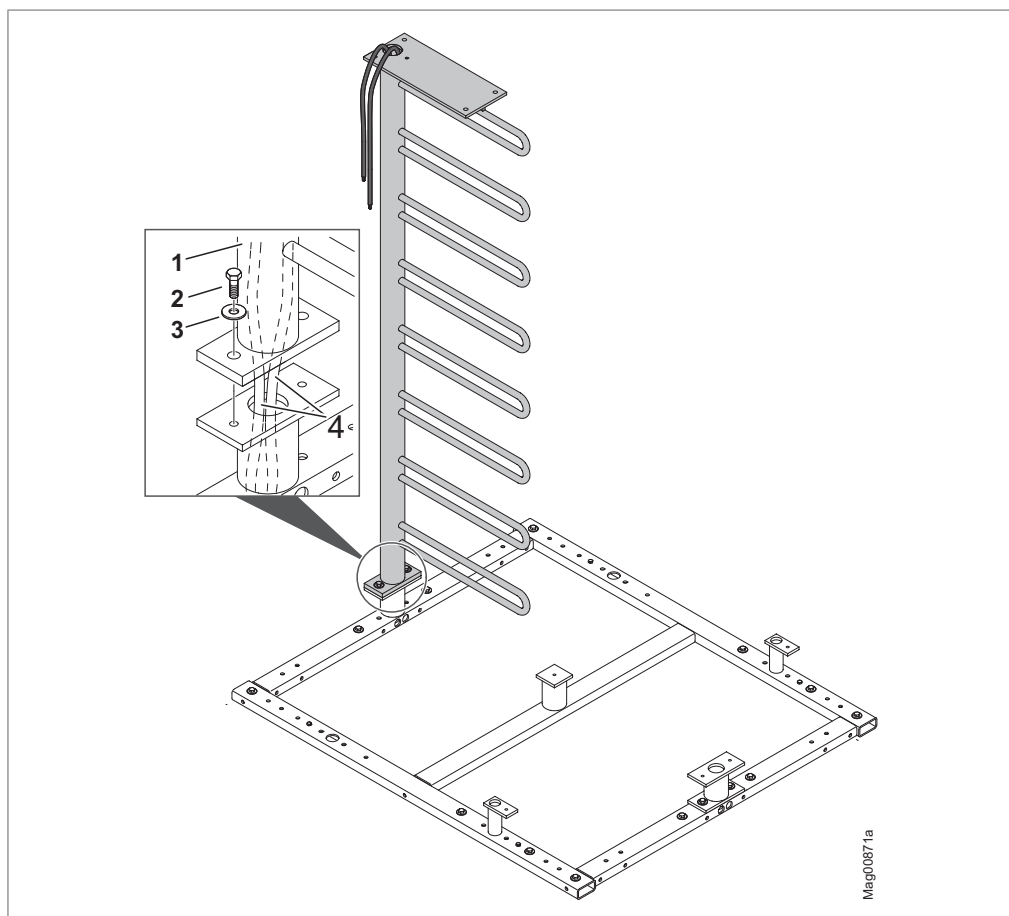
Fig. 22: Mounting the locking comb
