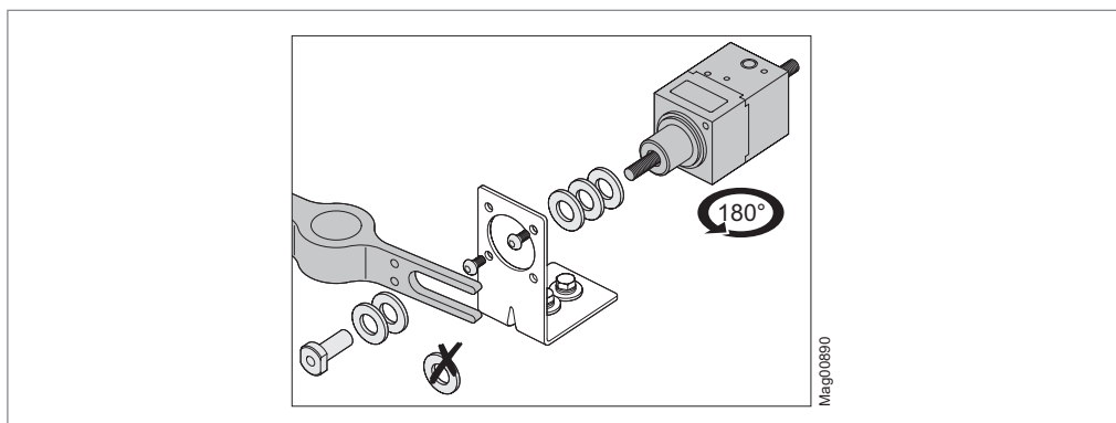
Fig. 61: Turn magnet, remove washer
