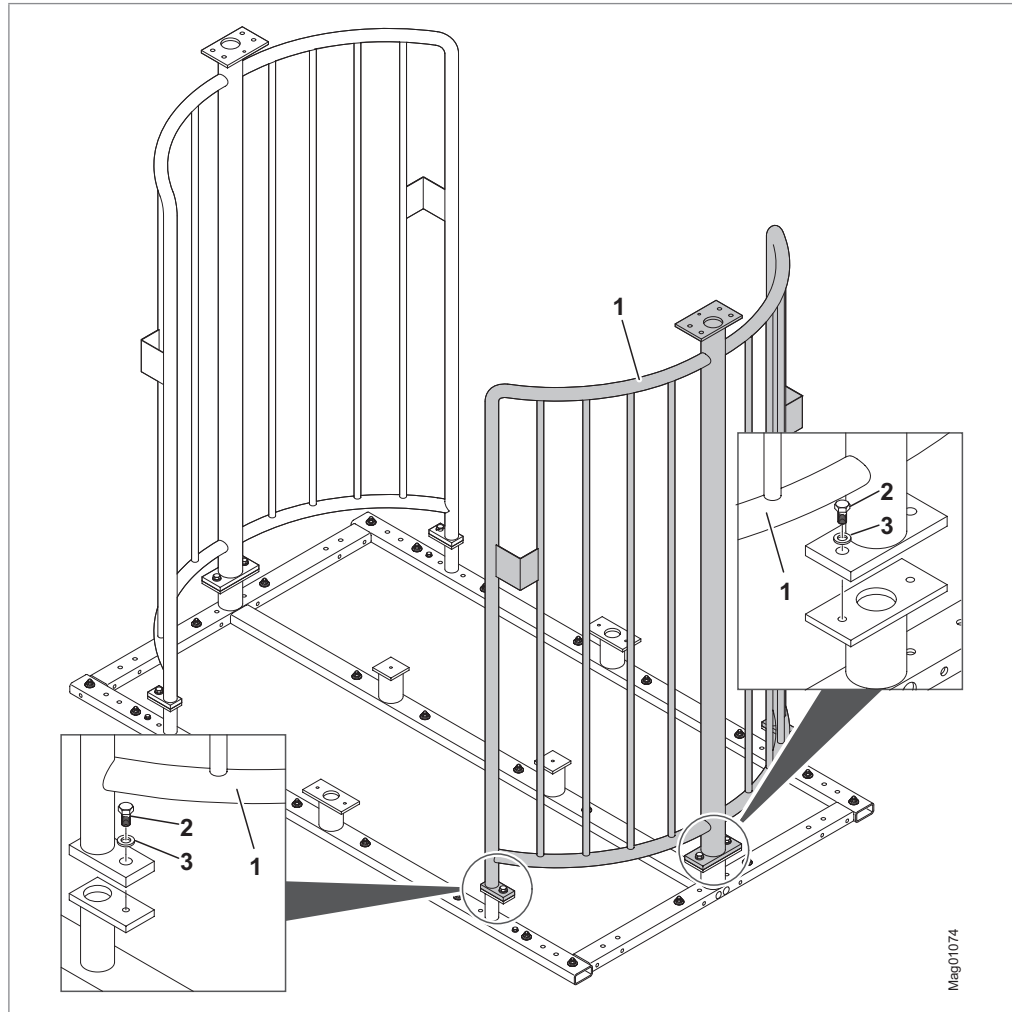
Fig. 34: Mounting the second cage half
