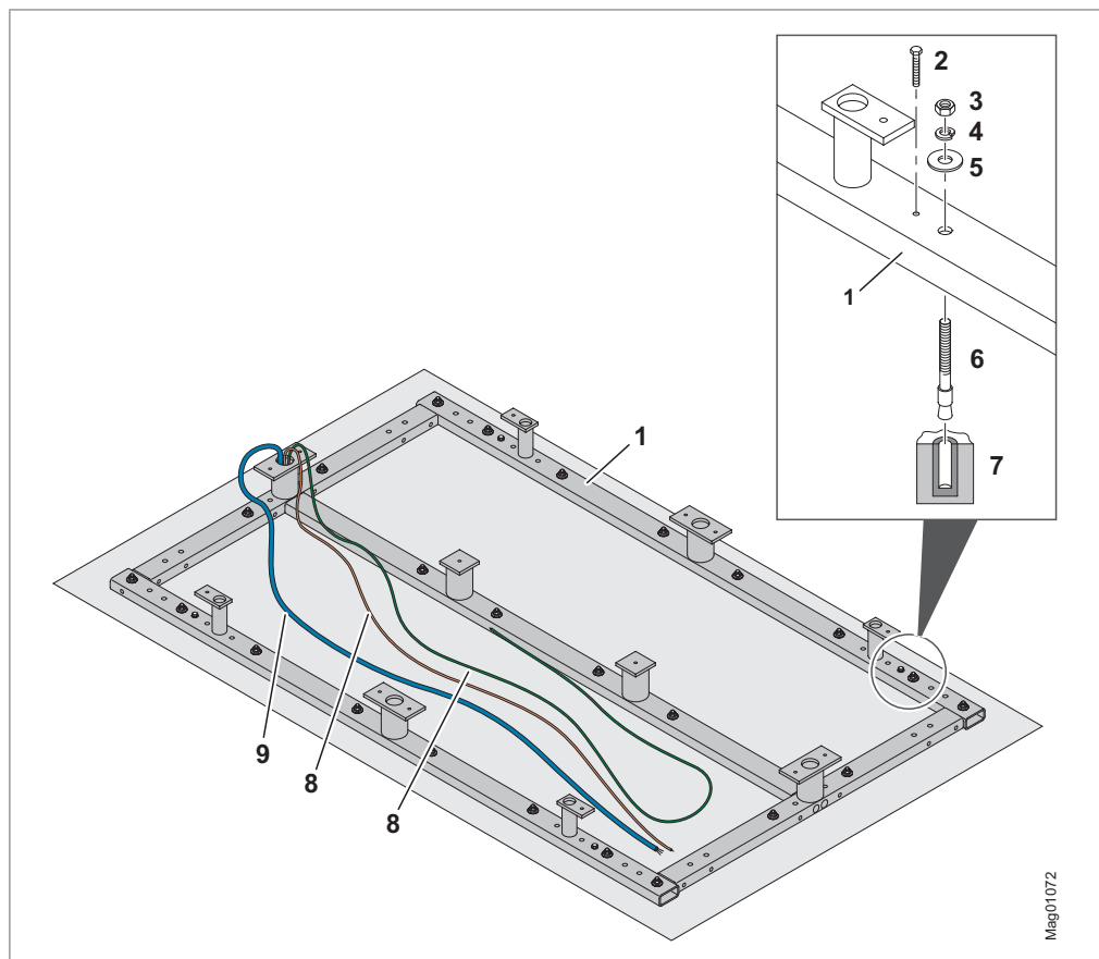
Fig. 32: Mounting the base frame FURA T5
