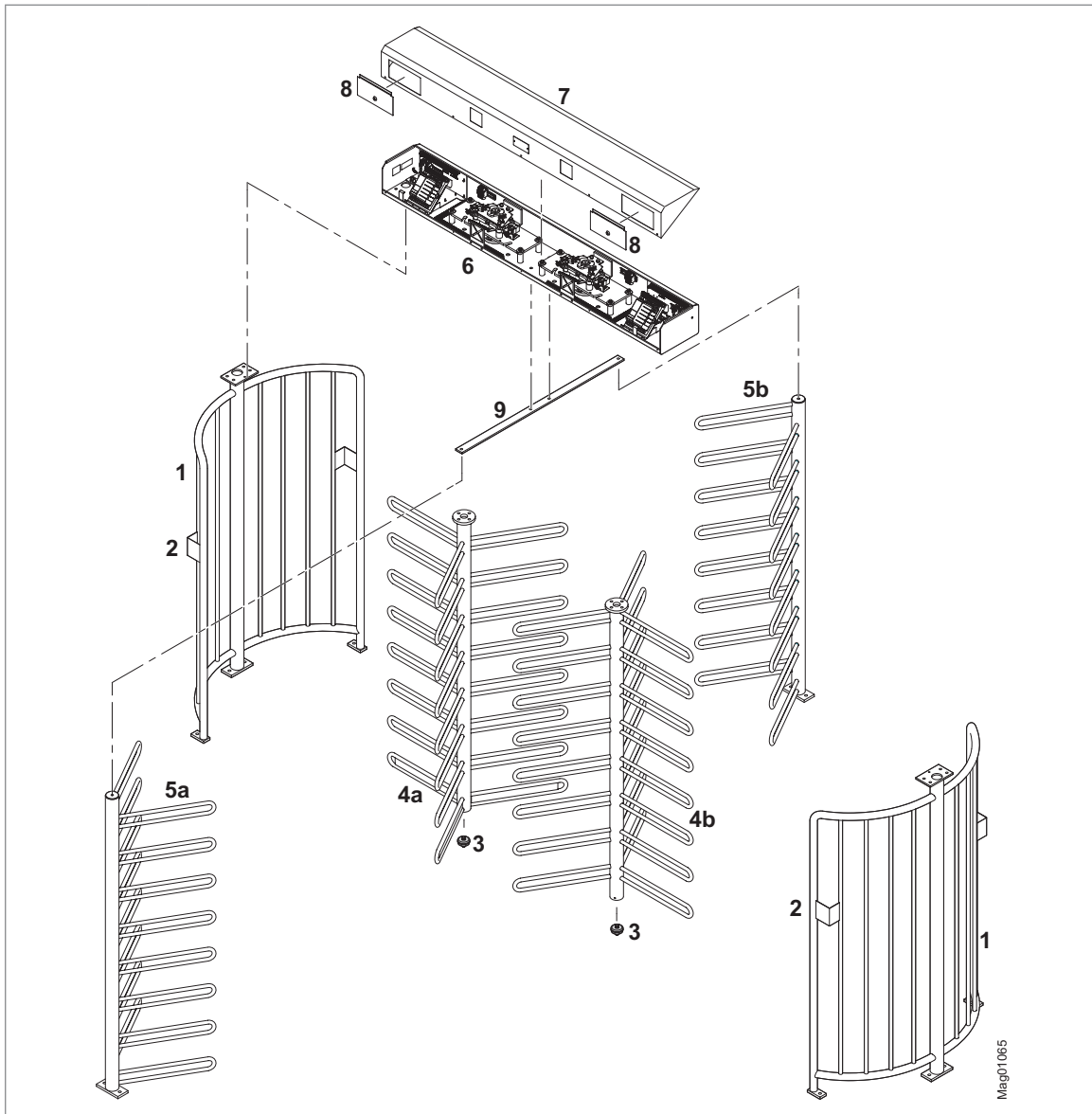
Fig. 8: Design "Full Height Turnstile MPT-353"
