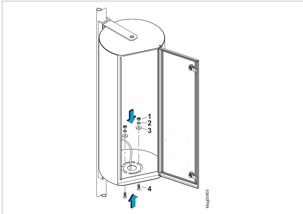
Fig. 51: Fixing the mounting pillar
