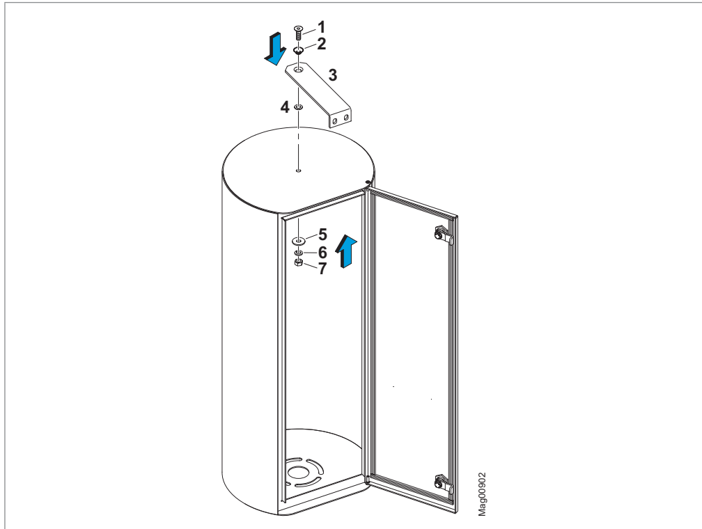
Fig. 48: Mounting the attachment angle
