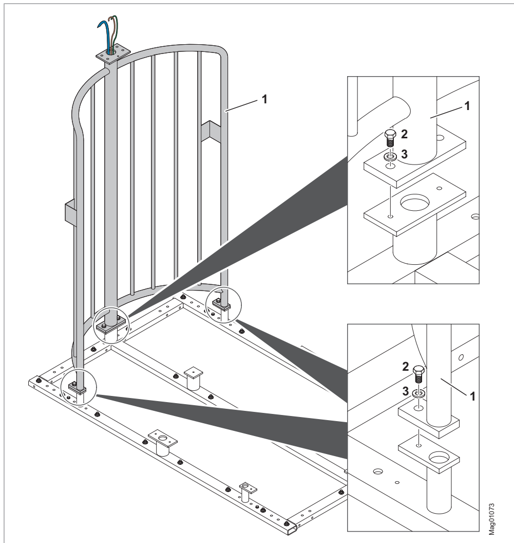
Fig. 33: Mounting the first cage half
