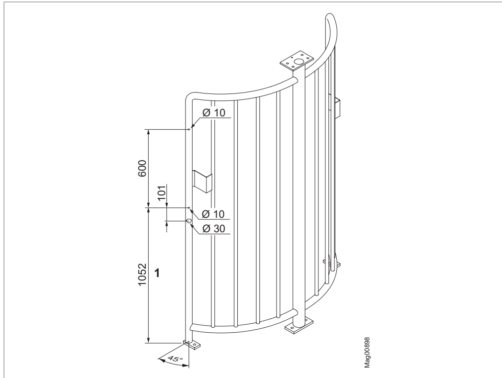
Fig. 44: Required holes mounting pillar (all dimensions in mm)
