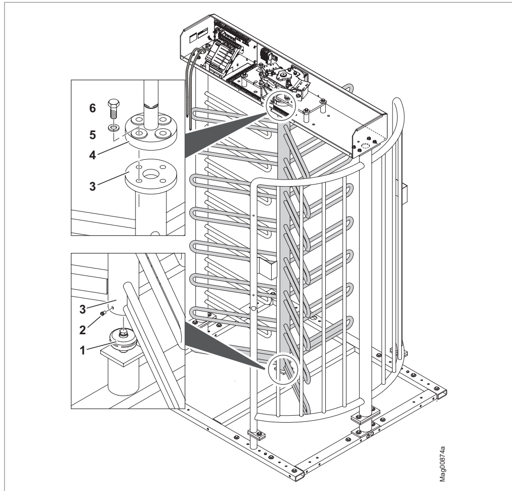
Fig. 26: Mounting the centre pillar
