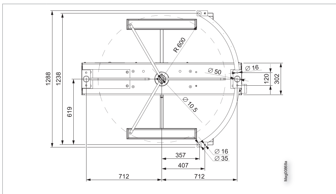
Fig. 3: Dimensions MPT-333 – view from below (dimensions in mm), illumination optional
