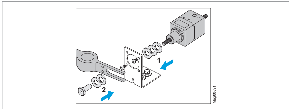
Fig. 62: Mount magnet, washers and union nut (normally open)
