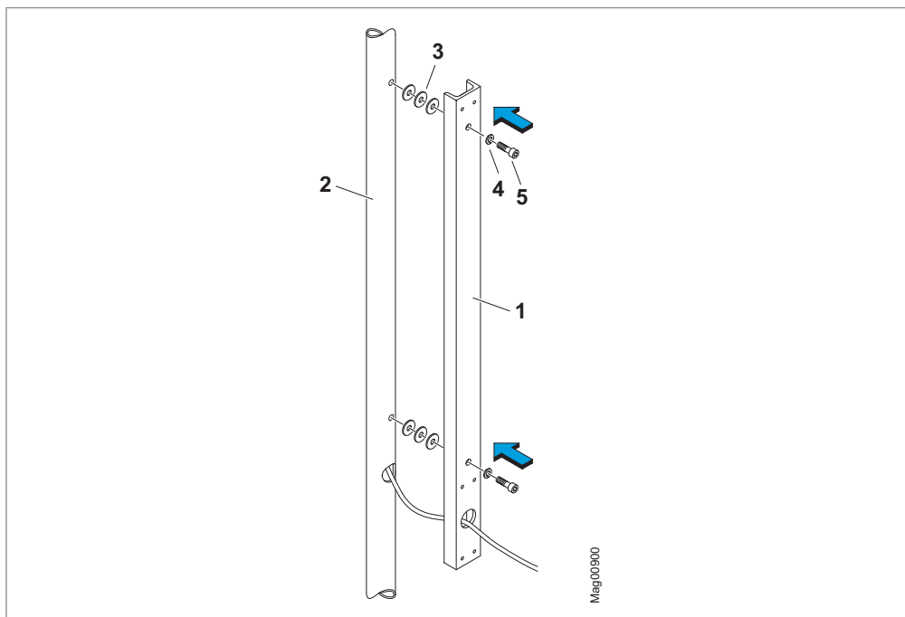
Fig. 46: Mounting the U-profile
