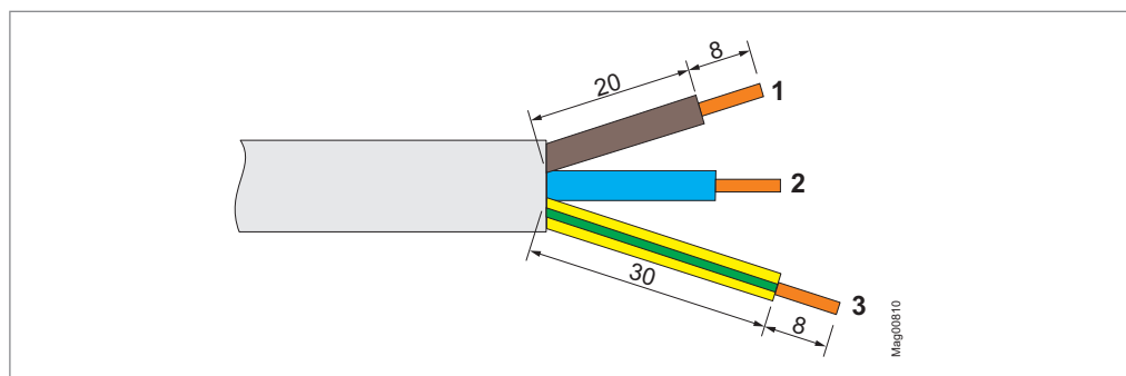
Fig. 53: Stripping (dimensions in mm)
