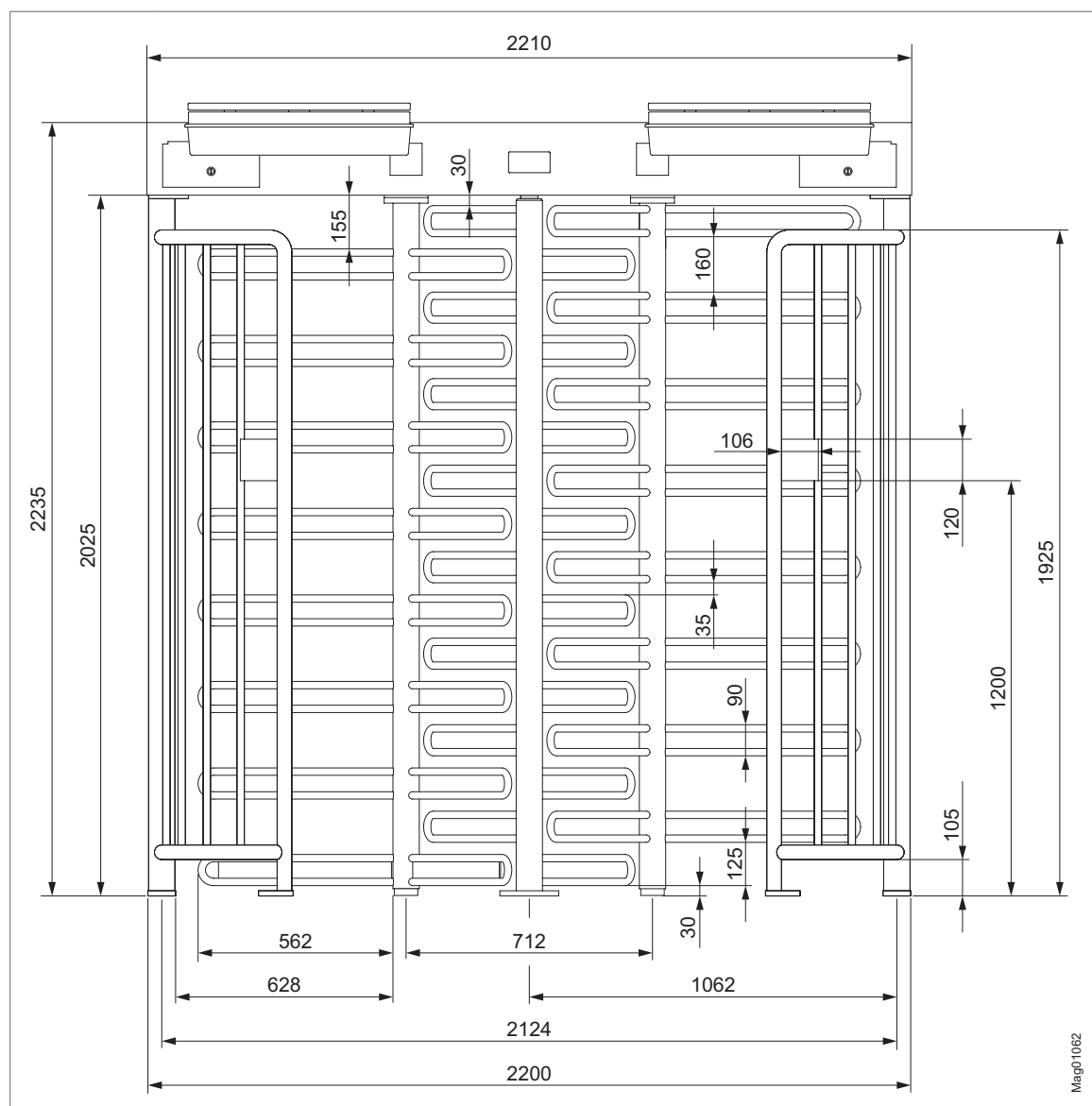
Fig. 4: Dimensions MPT-353 – front view (dimensions in mm), illumination optional
