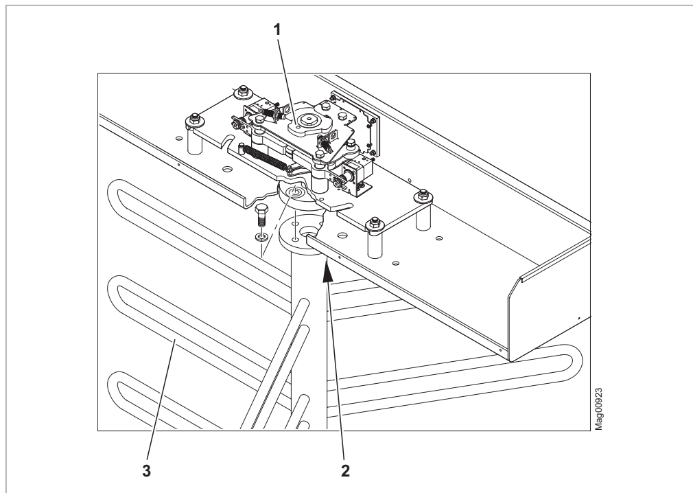
Fig. 40: Correct positioning of the locking unit – illustration shows version "Entrance side right"; in version "Entrance side left", the centre pillar is turned by 180°.
