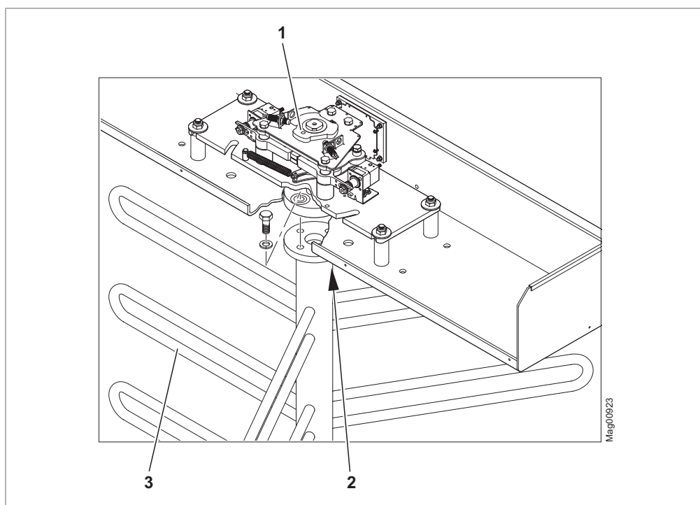
Fig. 27: Correct positioning of the locking unit – illustration shows version "Entrance side right"; in version "Entrance side left", the centre pillar is turned by 180°.
