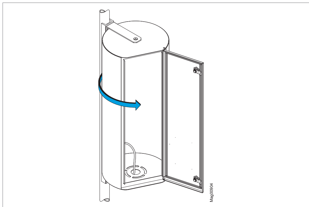
Fig. 50: Aligning the mounting pillar
