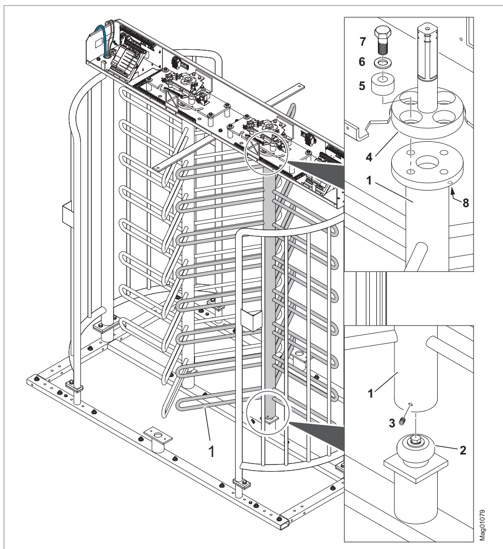
Fig. 39: Mounting the centre pillar without heel guard
